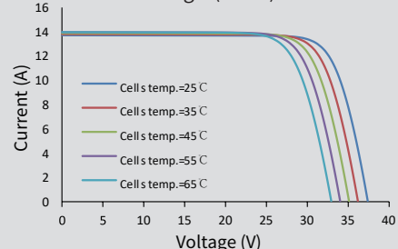
Current-Voltage (410W)
